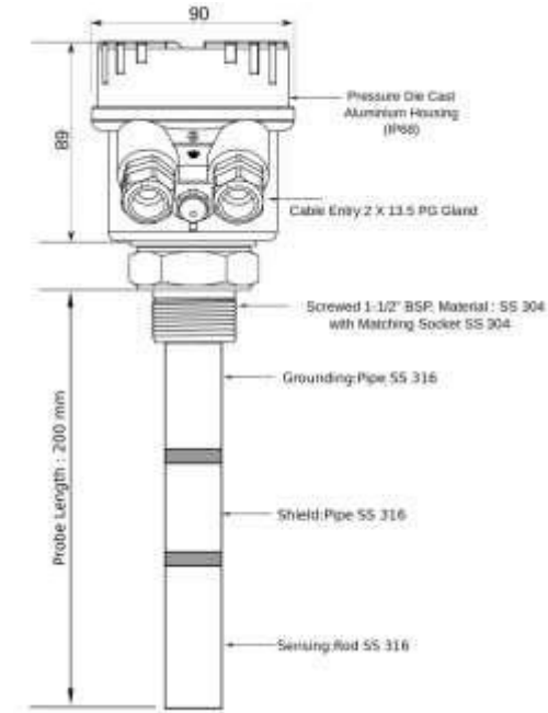
• GA Drawing
