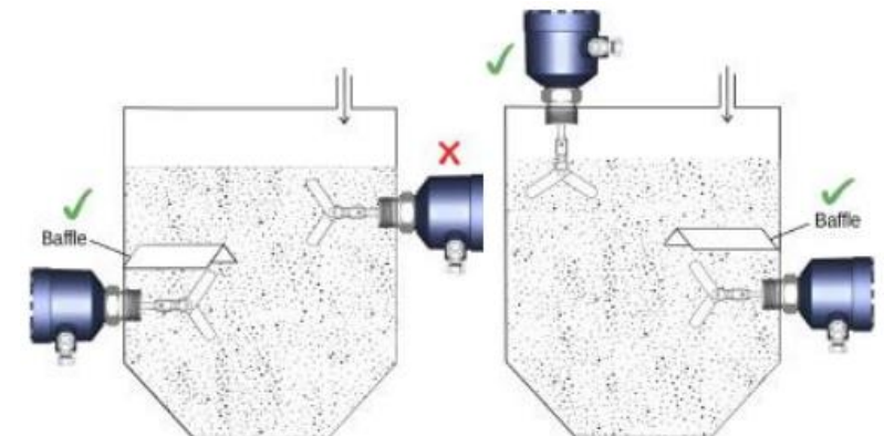
Figure 3: Correct Side Mounting
