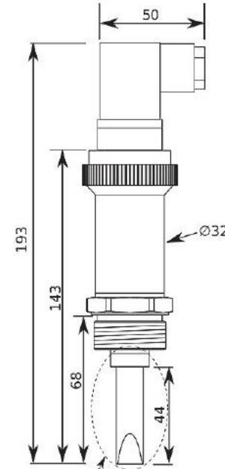
• GA Drawing
