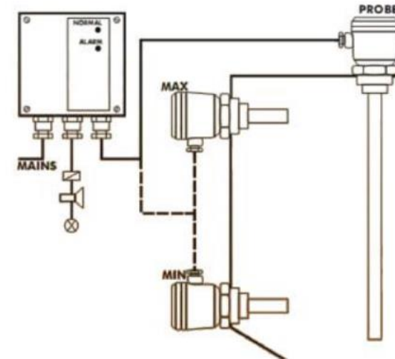
Figure 2: System Diagram
