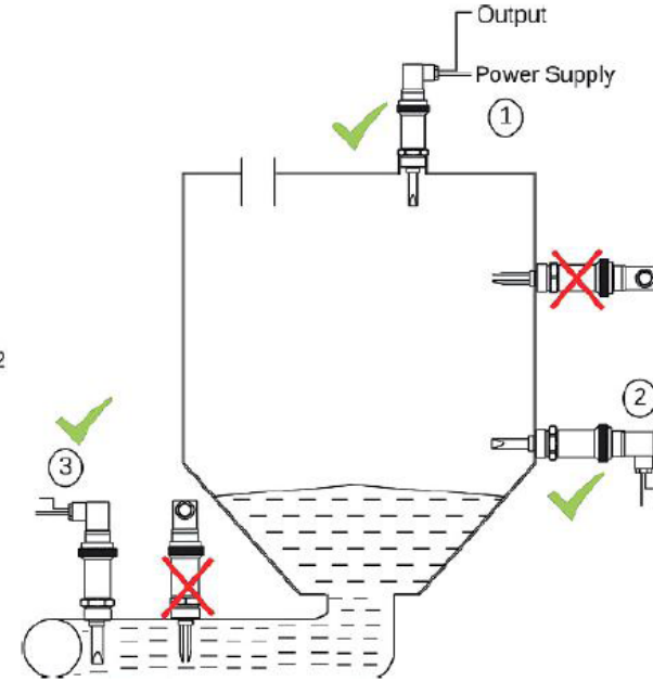
Figure 3: Installation Diagram
