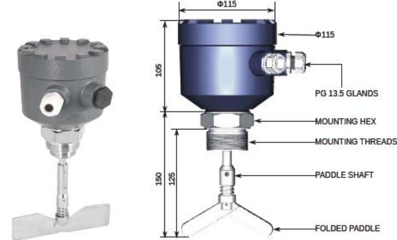
Figure 1: Parts of Orbit Paddle
